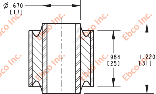
SECTION X-X
