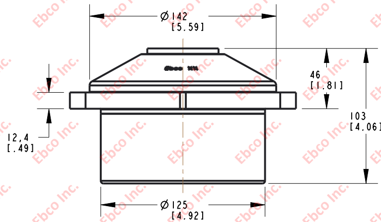
INSTALLATION DIMENSIONS
