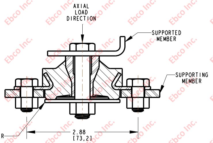
INSTALLATION VIEW (Shown under no load)
