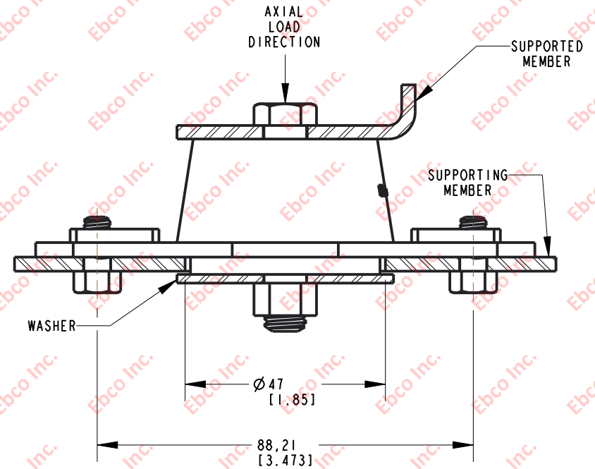
INSTALLATION VIEW (Shown under no load)
