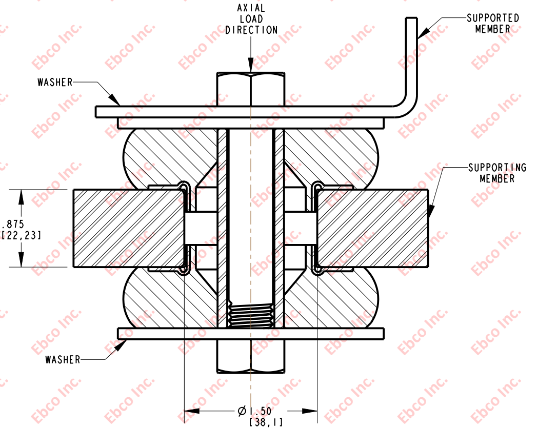
INSTALLATION VIEW (Shown under no load)
