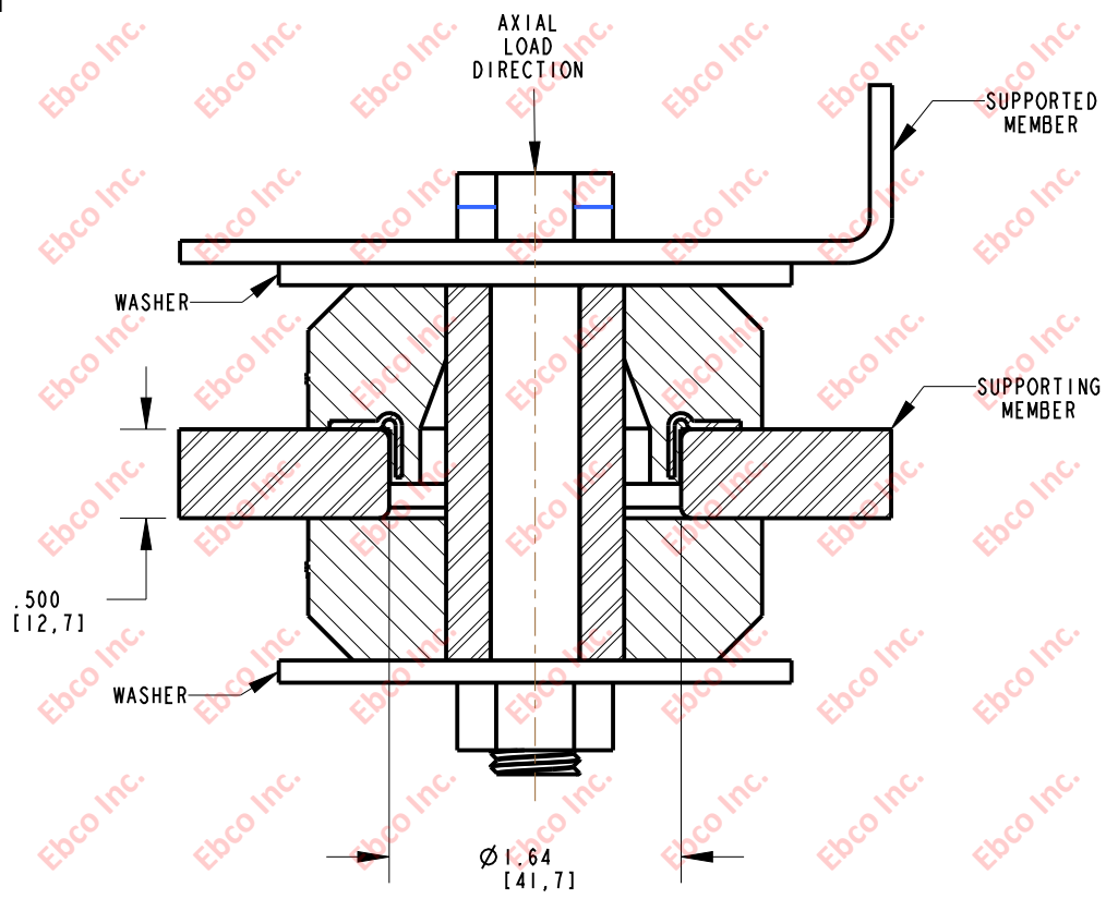
INSTALLATION DIMENSIONS
