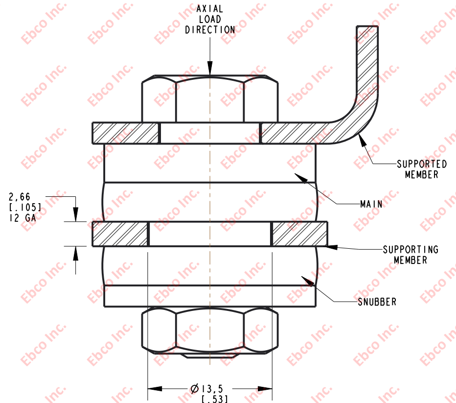
INSTALLATION VIEW (Shown under no load)
