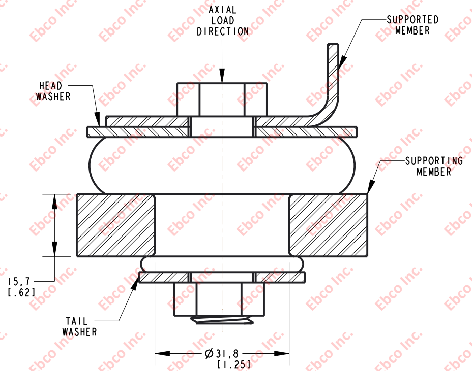
INSTALLATION DIMENSIONS
