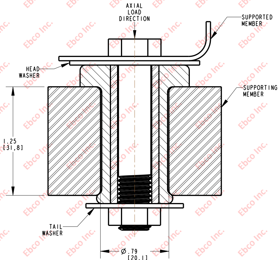
INSTALLATION DIMENSIONS
