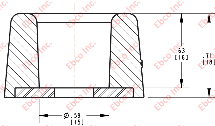
SECTION X-X
